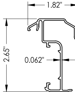
"TRADITIONAL" PROFILE
