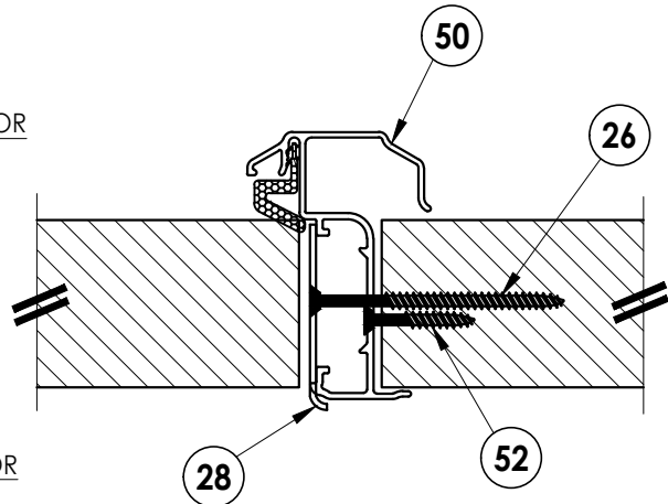
5 5 HORIZONTAL CROSS SECTION Inswing shown (Outswing similar)
