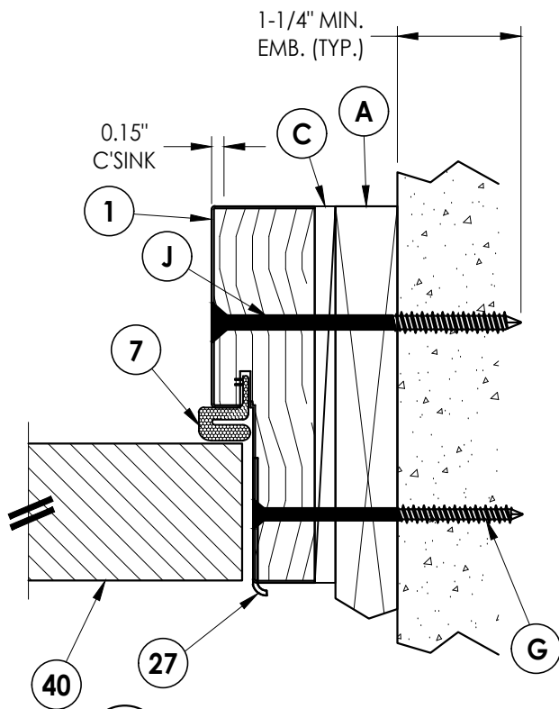
4 5 HORIZONTAL CROSS SECTION Inswing shown (Outswing similar) 1X Buck Construction
