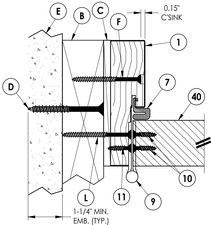
1 5 HORIZONTAL CROSS SECTION Inswing shown (Outswing similar) 2X Buck Construction
