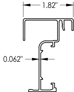
"MODERN" PROFILE
